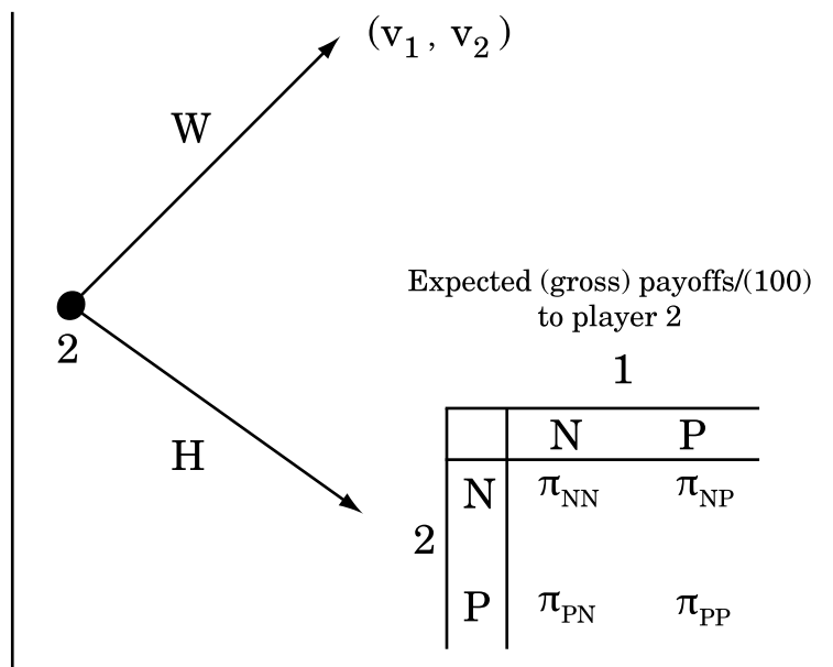
Figure 2: Payoff Structure
